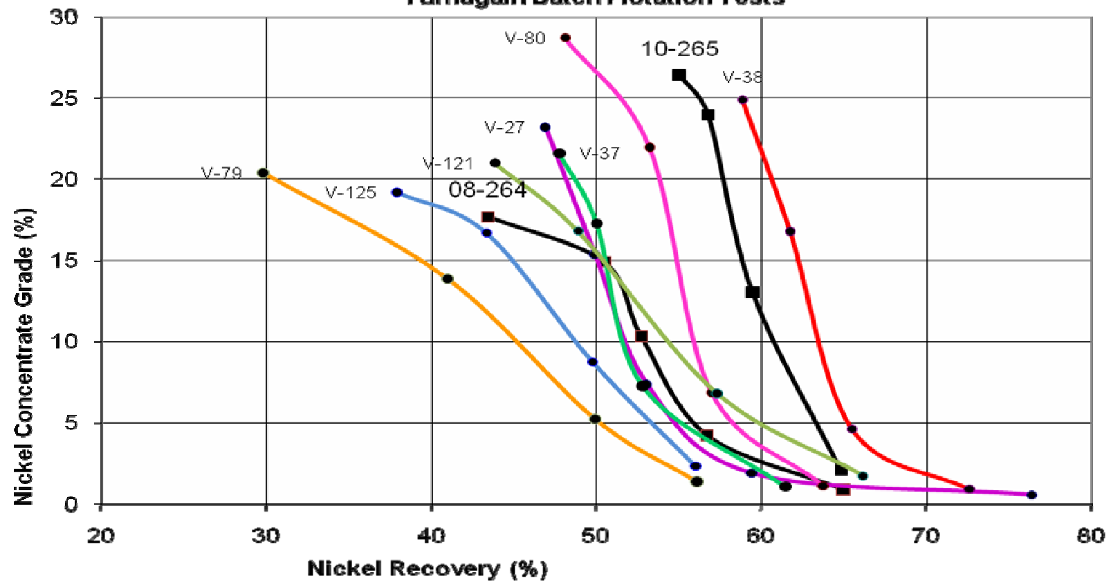
Figure 1: Nickel Concentrate Grade vs Recovery Turnagain Batch Flotation Tests
