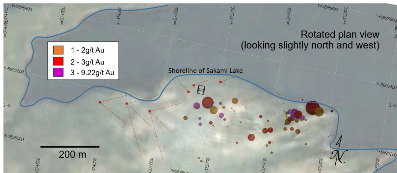
Figure 1. Oblique image of Zone 25 showing the distribution of mineralized intervals created using a 1g/t lower limit and shown as spheres according to the thickness. Red traces represent the planned drilling.
