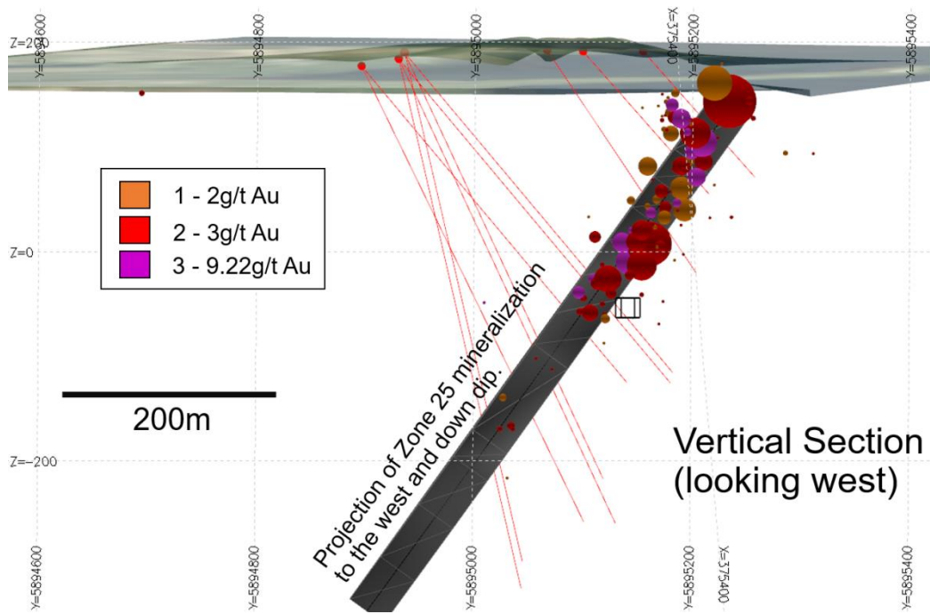
Figure 2. Vertical section looking west, showing the proposed drill traces in red with respect to the possible extensions to Zone 25 (grey polygon).
