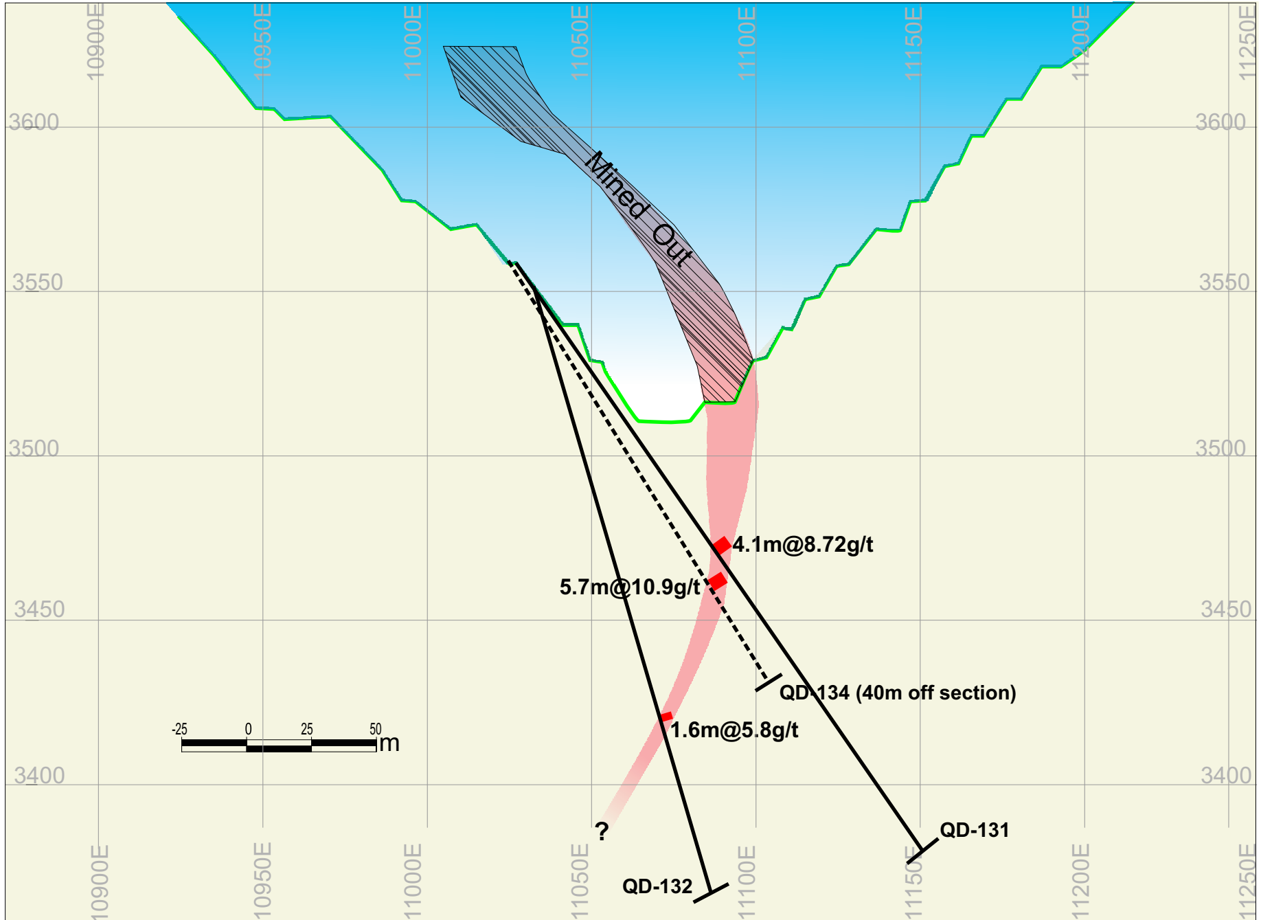
Figure 3 Qinglongtan Cross Section Showing QD-131 and QD-132
