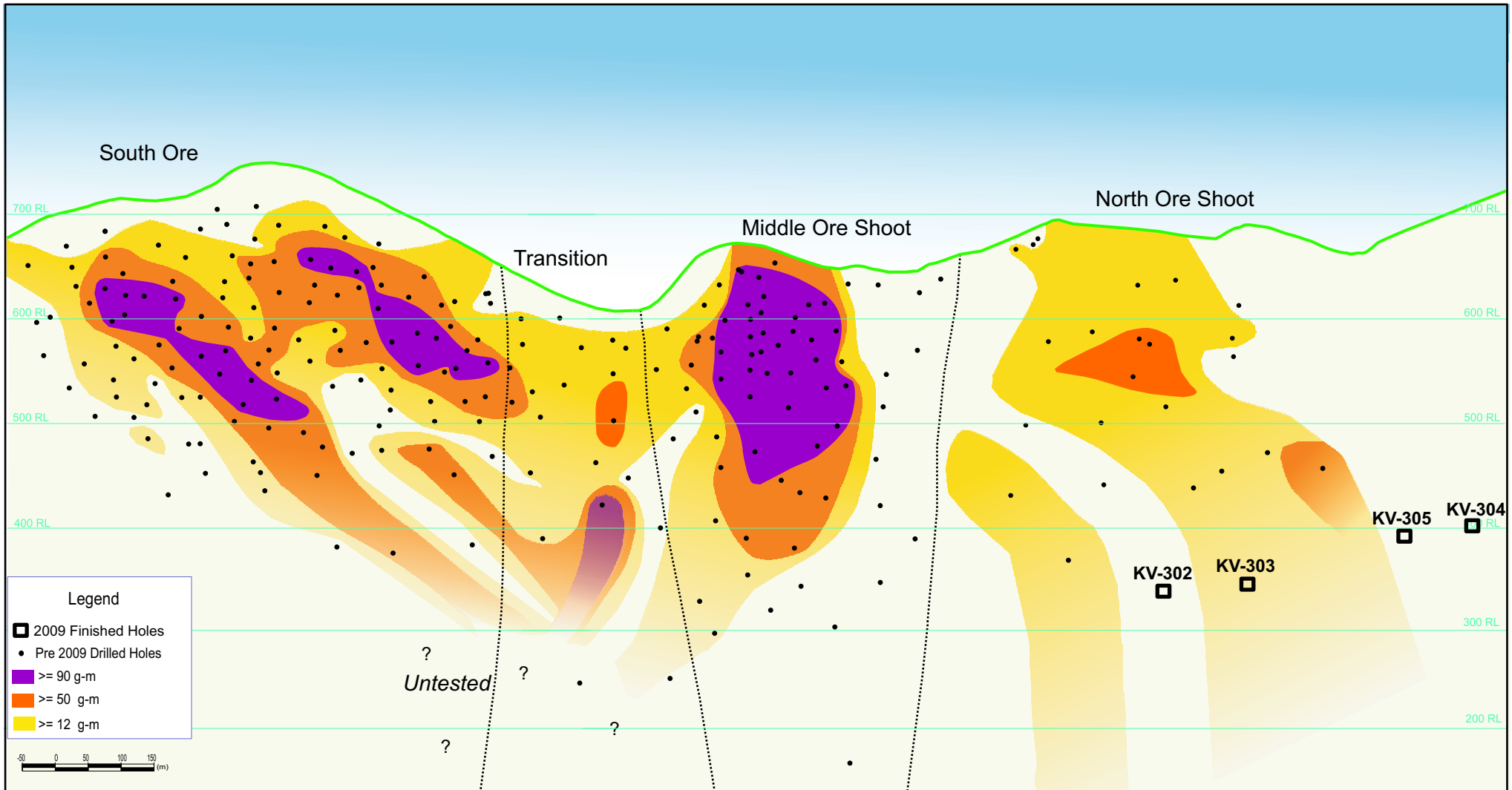
Figure 2 Efemçukuru North Ore Shoot Longitudinal Section Looking Southwest
