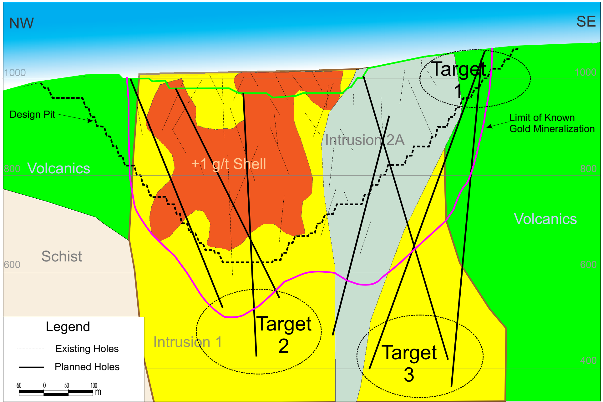
Figure 1 Kisladag Section Showing 2009 Planned Drill Holes
