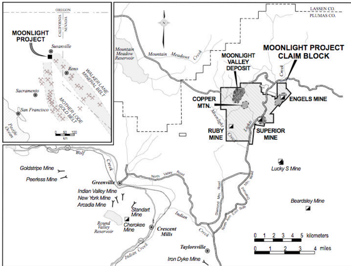
Figure 1 - Moonlight Project Showing Copper Deposits with Location Inset Map
