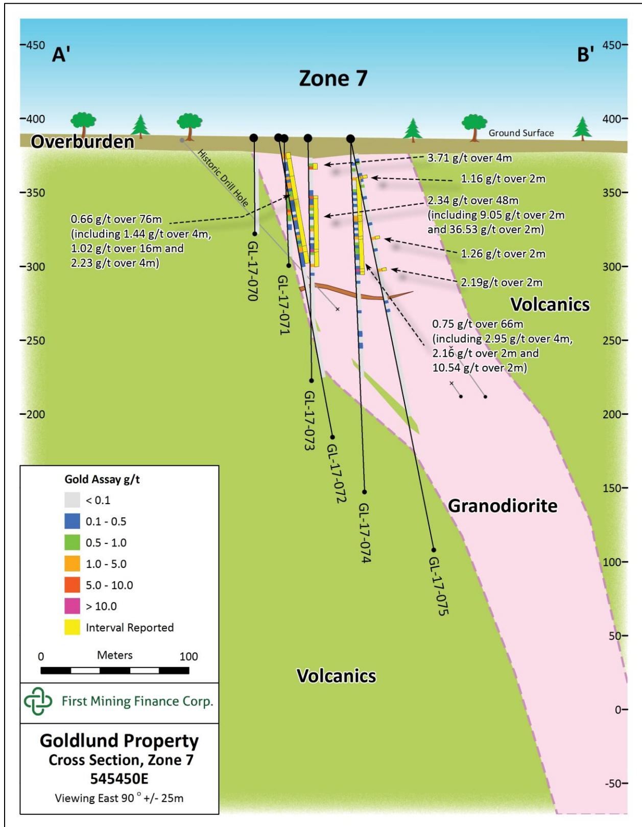
Figure 2. Cross-Section through the Goldlund Project
