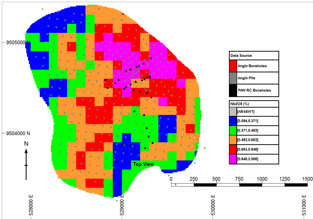
Figure 2 – Surface Plan View of Resource Model Showing Continuity of High Grade Zone
