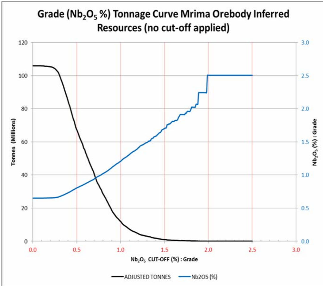
Figure 1 – Grade Tonnage Curve for the Niobium Mineral Resource Estimate - Mrima Hill Deposit
