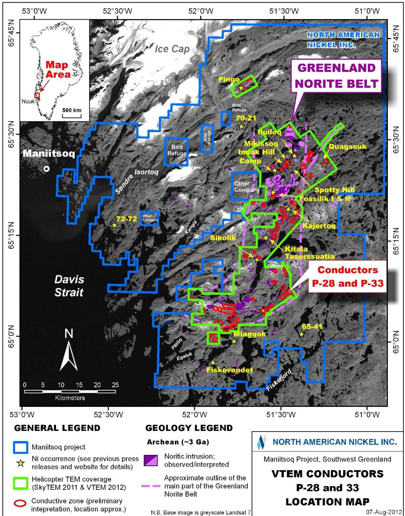
Figure 1: Landsat image of the Maniitsoq project showing the location of VTEM conductors P-28 and P-33.
