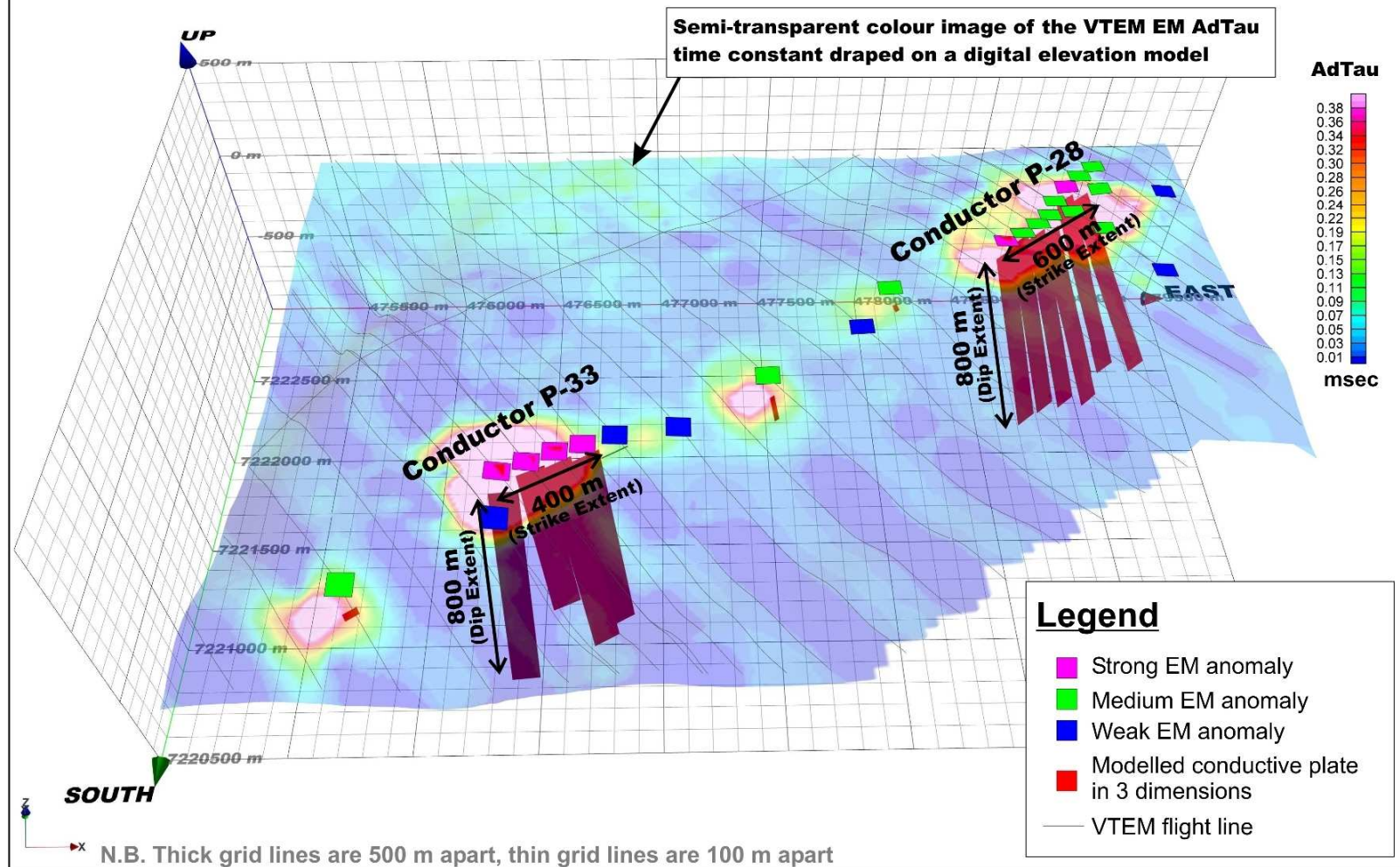
Figure 2: Example of three-dimensional EM modeling for two conductors in the east central part of the Greenland Norite Belt. See Figure 1 for location of conductors.
