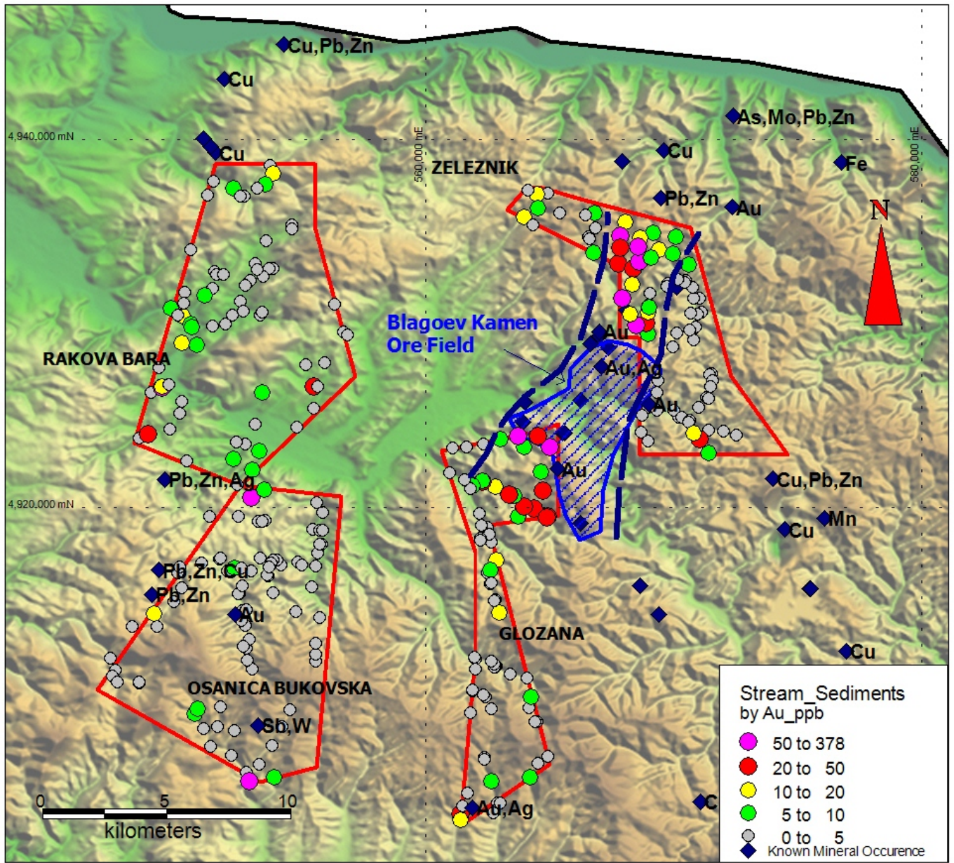
Figure 1. Stream sediment Au results.
