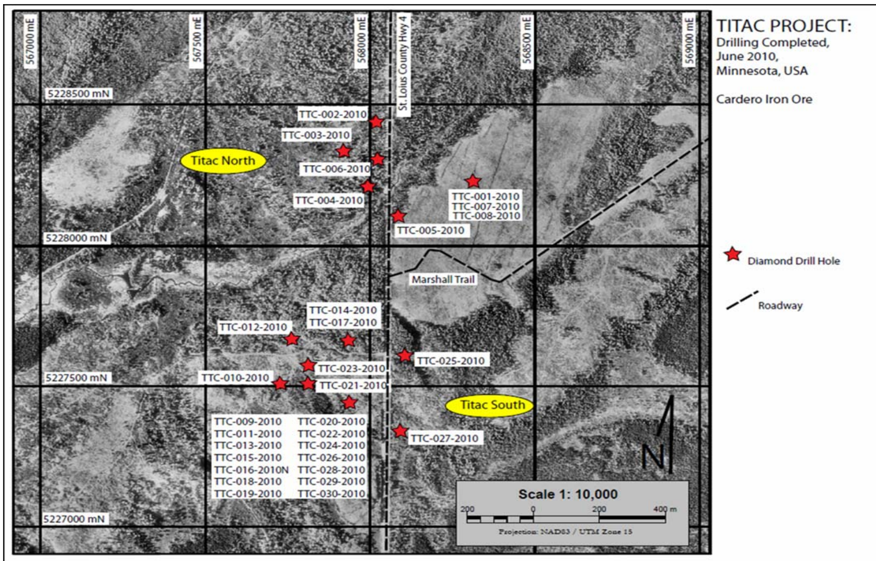
Figure 1: Drilling completed on TiTac project – some platforms have multiple drillholes
