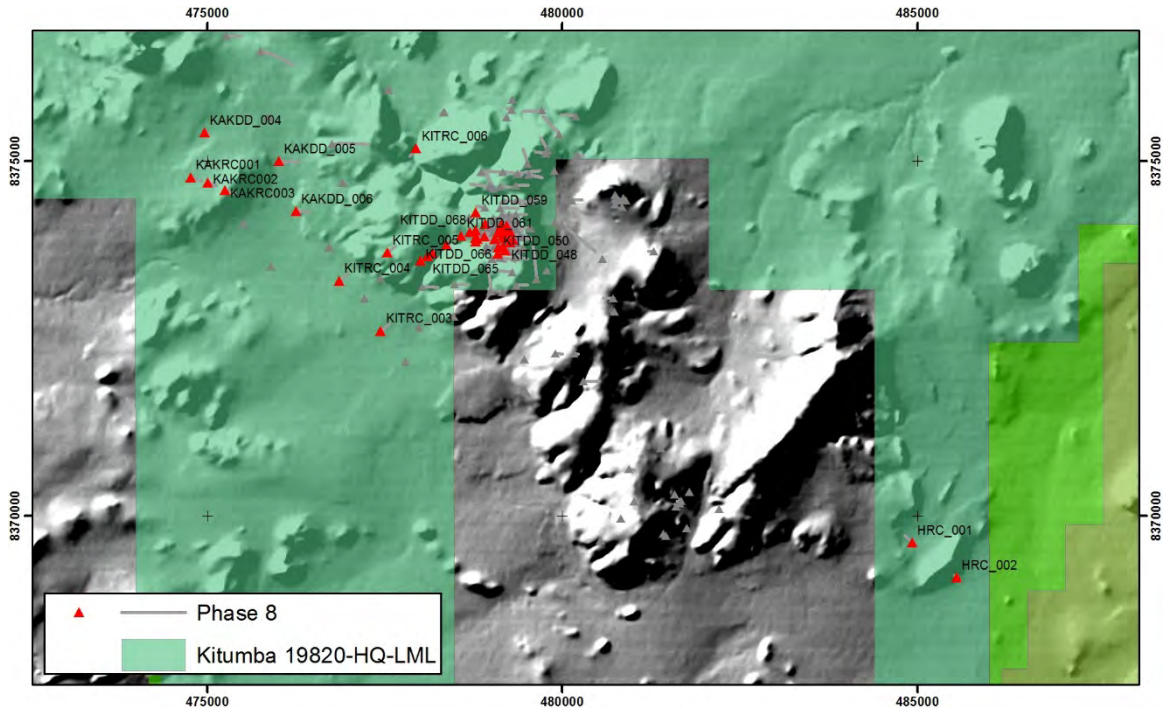
Figure 2. RC and sterilisation drill hole location plan showing collar locations and company tenure on hill shaded elevation model.
