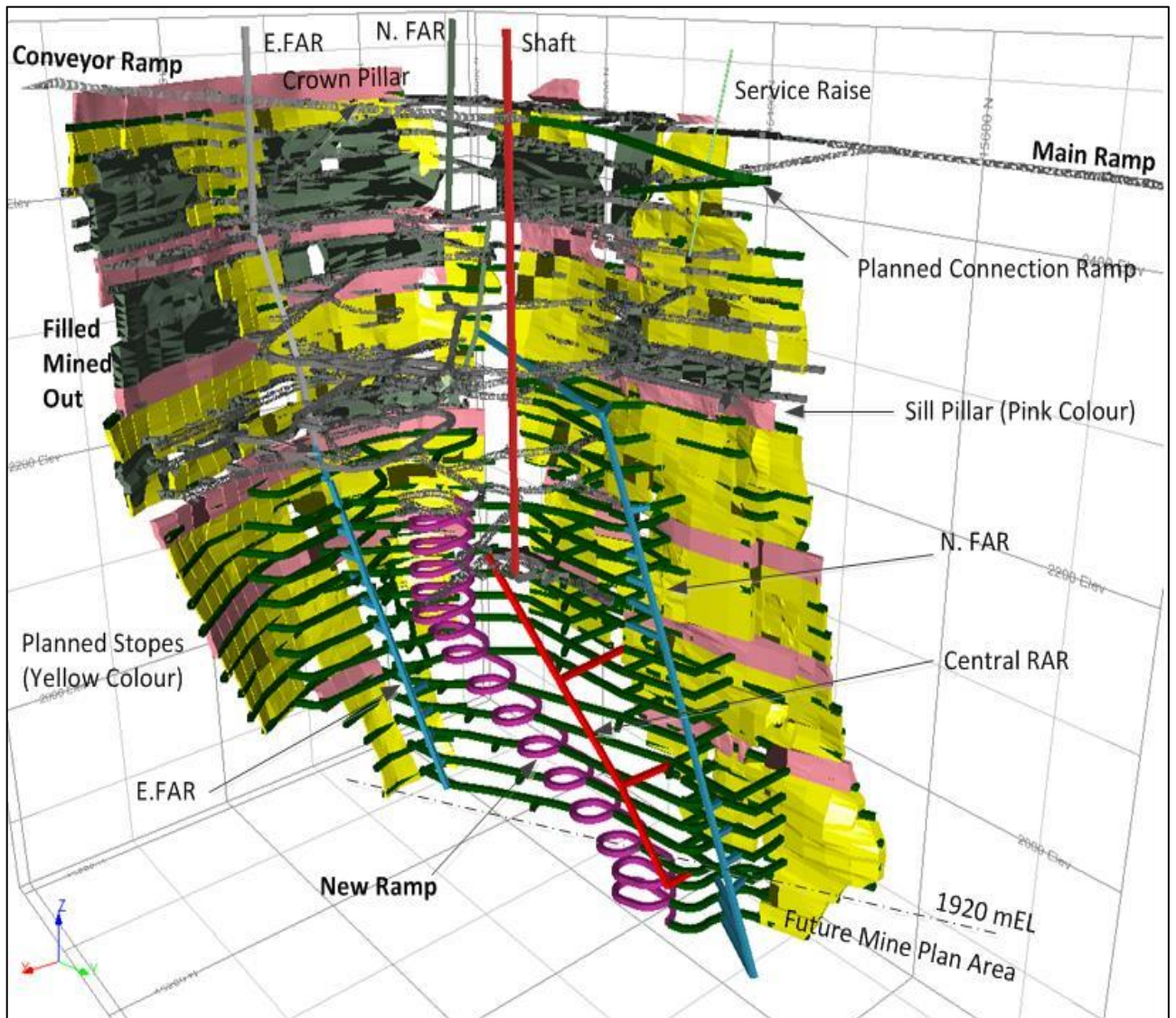
Figure 1: 3D Mine Model Isometric View of the Caribou Mine Plan Looking Southwest (Yellow represents Planned Stopes; Pink represents Sill Pillar; Gray represents Previously Mines Stopes and Fill)
