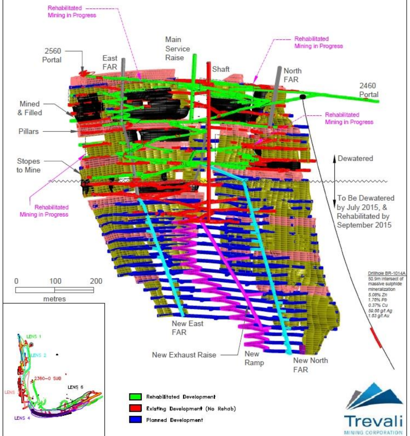
Figure 3: Caribou Mine underground production and development plan. Note resources extend below lowest levels illustrated.
