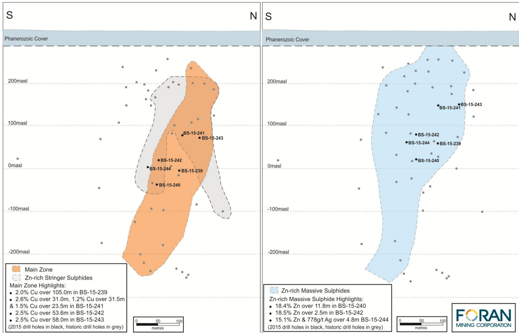
Figure 2. Longitudinal Sections of the Main Zone, Zn-rich Stringer Sulphides and Zn-rich Massive Sulphides (looking northwest).
