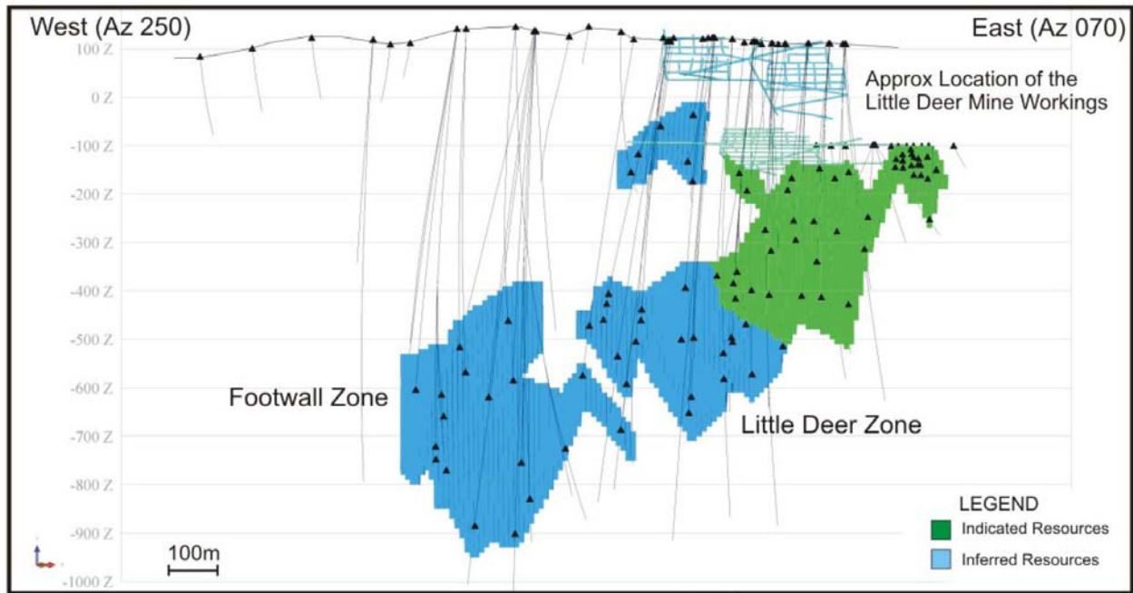
Figure 1: Longitudinal View, Little Deer Copper Deposit Looking NNW (after Scott Wilson RPA, September 30, 2010) (Green – Indicated Resources; Blue – Inferred Resources).
