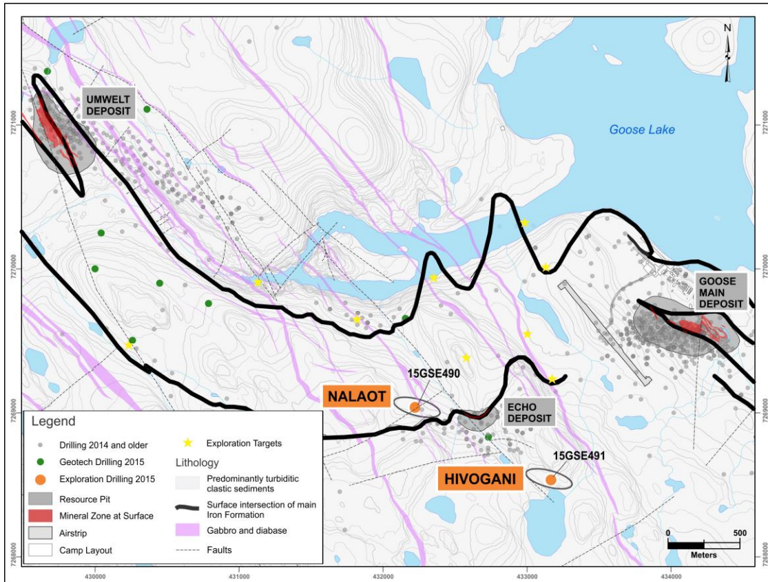
Figure 1: Project Geology Map with 2015 Exploration Drillhole Collars and Target Areas.
