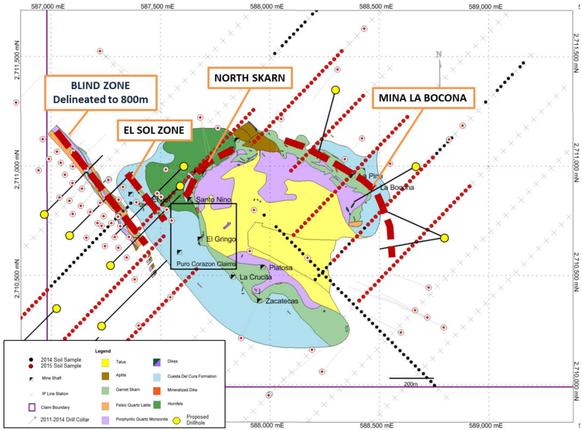
Figure 1: Initial drill plan and soil sample stations for the 2015 exploration program in the area of the Cerro at the Cerro Las Minitas Property. The proposed drill holes are indicated in yellow.
