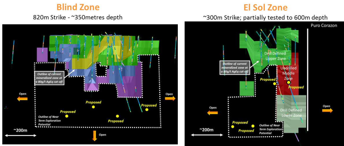
Figure 2: Projected pierce points for 2015 drilling on the Blind and El Sol zones. Drilling success will significantly expand the extent of these mineralized zones.
