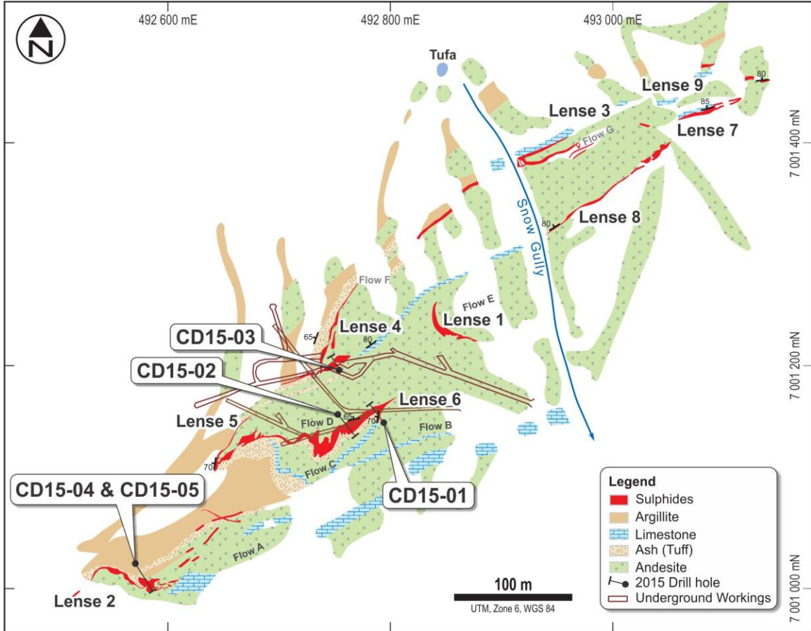
Figure 1. Geology around the nine known lenses of mineralisation at the Caribou Dome Copper Project, together with surface traces of underground development and locations of recent drill holes.
