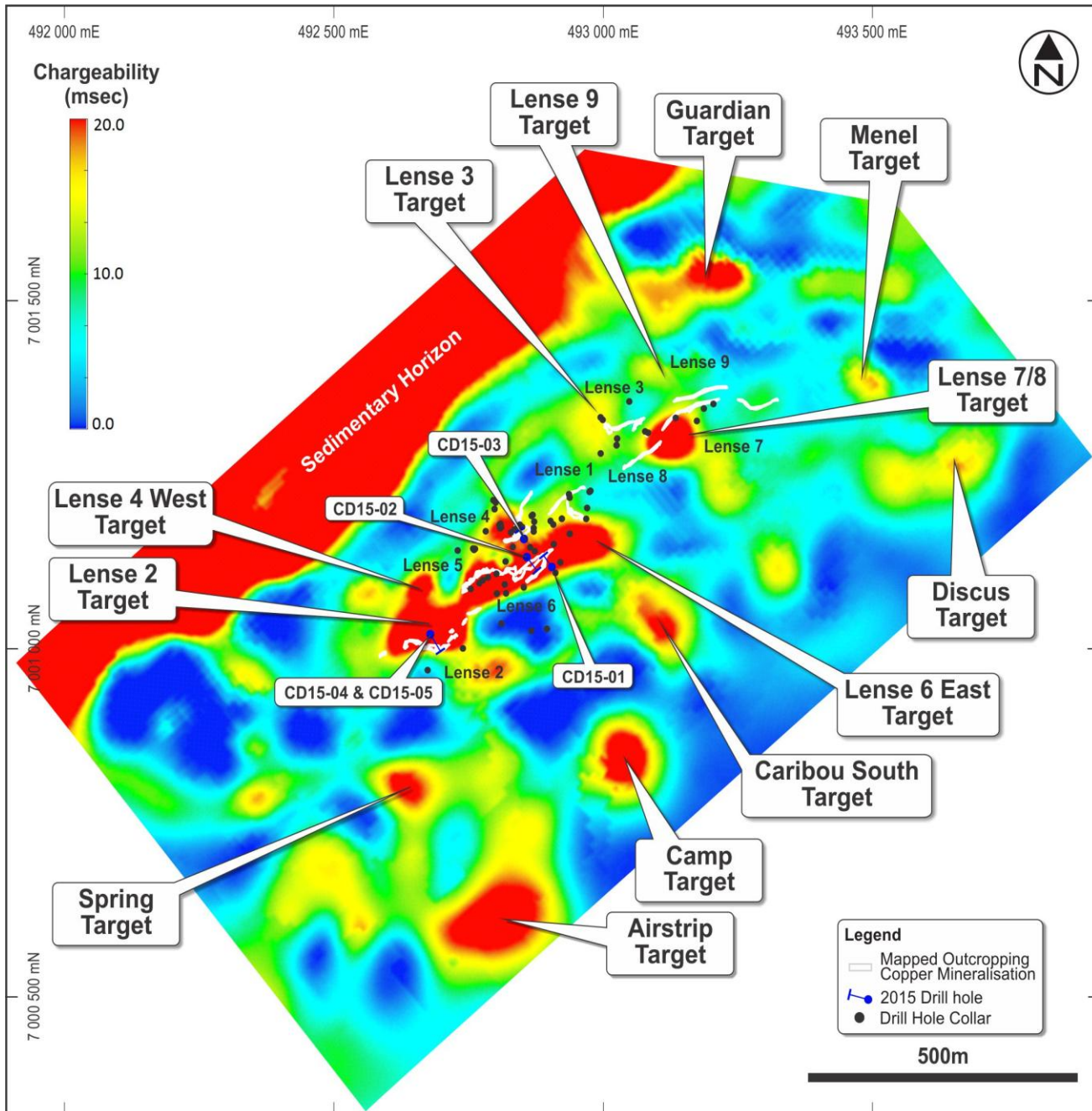
Figure 2. “100-metre depth slice” of inverted 3DIP chargeability data – showing the chargeability of the modelled source of 3DIP anomalies, 100 metres below the surface, together with labels highlighting higher-priority targets that will be evaluated further. (It is noted that the sources of some of the highest priority targets are modelled to be greater than and less than 100 metres deep – so not all targets appear as intense anomalies in the 100m depth slice plan above).
