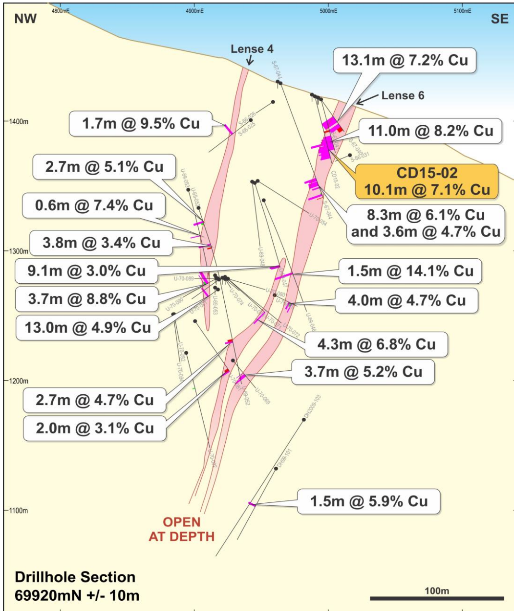
Figure 3. Cross section showing mineralisation in drill hole CD15-02 and other adjacent historic drill holes.
