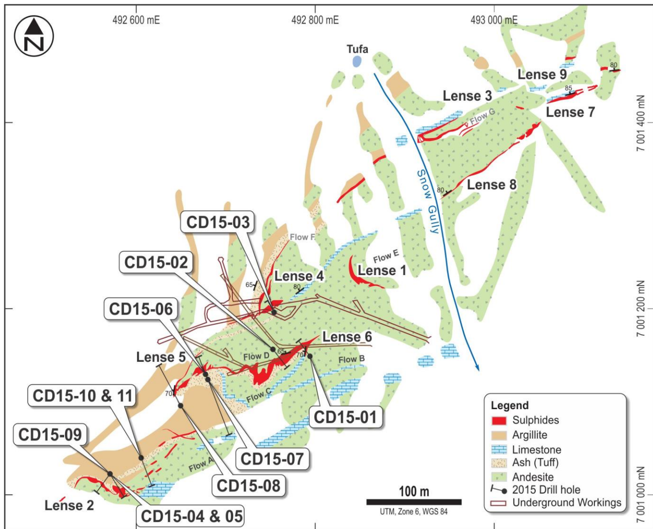
Figure 1. Geology around the nine known lenses of mineralisation at the Caribou Dome Copper Project, together with surface traces of underground development and locations of Coventry's recent drill holes.
