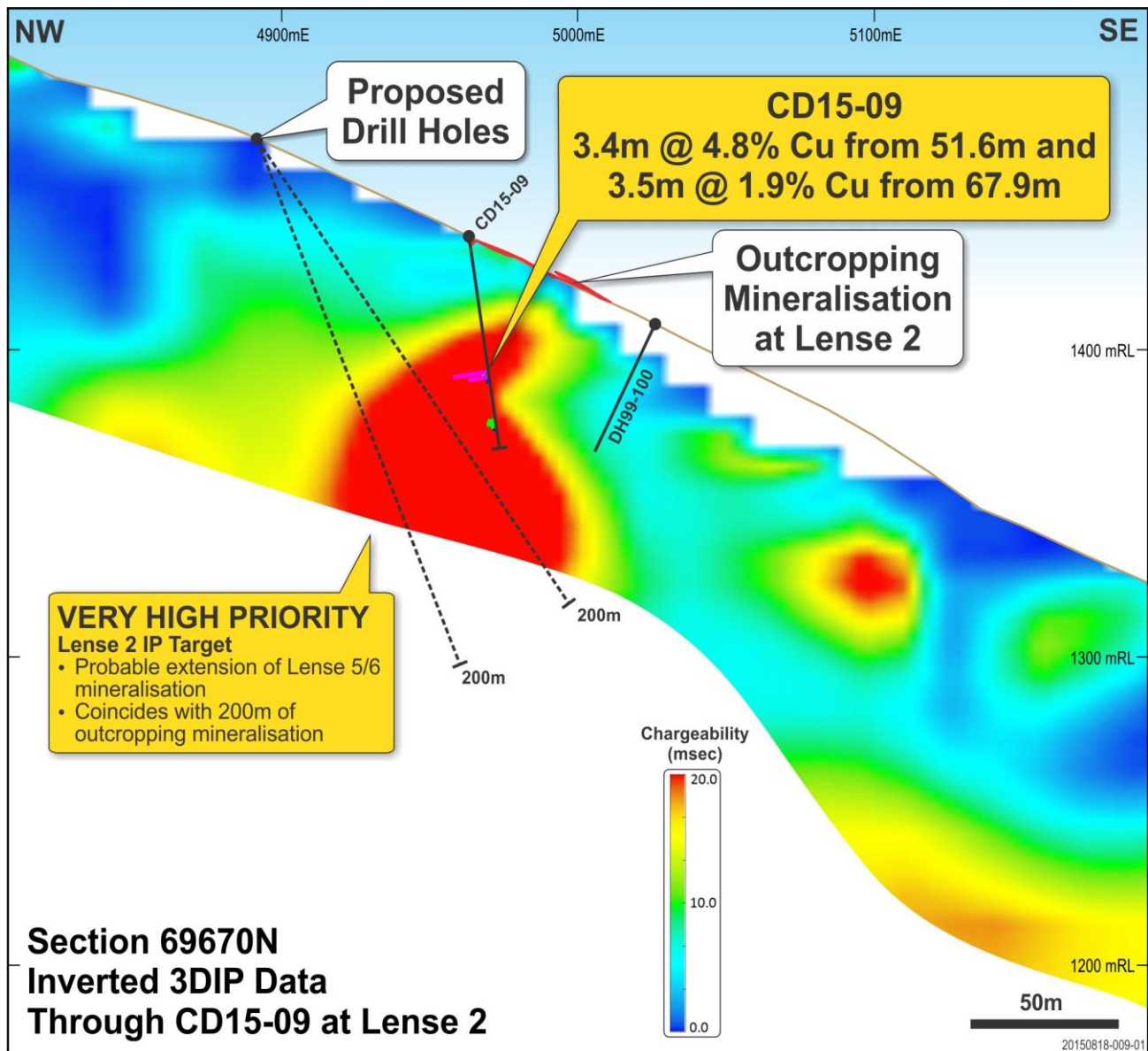
Figure 2. Cross section of inverted 3DIP data through the central portion of Lense 2, showing mineralisation intersected in drill hole CD15-09. This mineralisation coincides with a narrow portion of a strong IP anomaly that broadens and strengthens at depth. Deeper drilling will be undertaken during the Company's ongoing 4,000m exploration drilling program to help determine whether thicker and/or higher-grade extensions of this mineralisation coincide with this anomalism.
