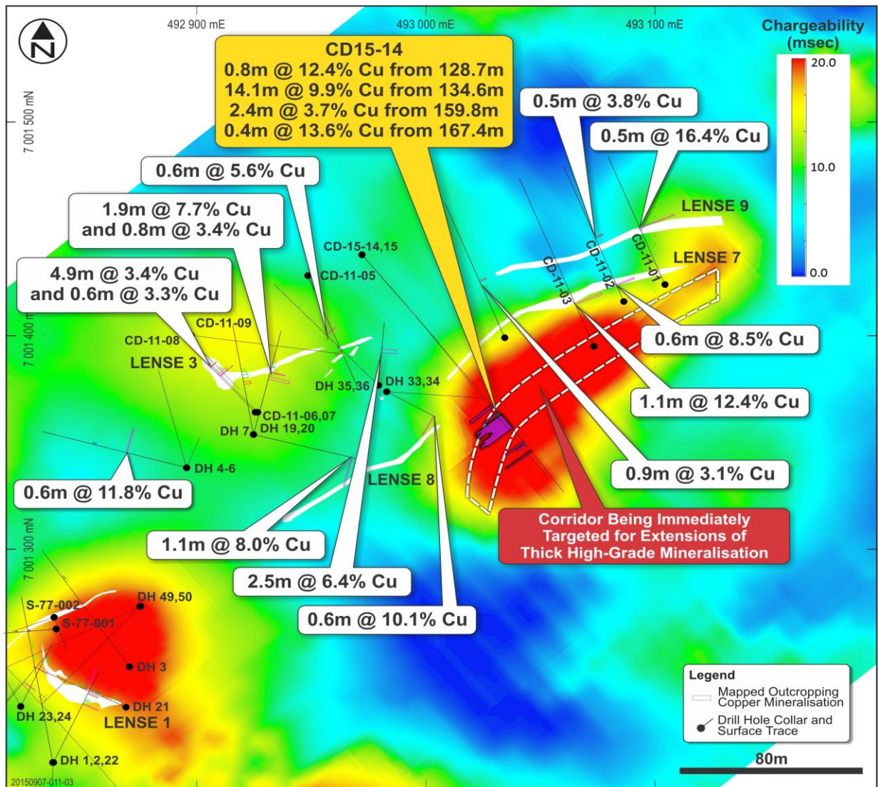
Figure 1. "50-metre depth slice" of inverted IP chargeability data at the Lense 7/8 Target – showing the chargeability of the modelled source of IP anomalies, 50 metres below the surface, together with previous drilling in the vicinity. (It is noted that the 50m depth slice doesn't highlight the entire length of the Lense 7/8 IP Target, as the depth of this anomaly varies along strike).
