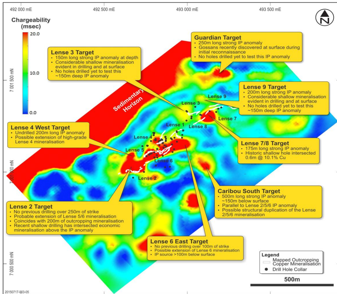
Figure 4. “100-metre depth slice” of inverted 3DIP chargeability data – showing the chargeability of the modelled source of 3DIP anomalies, 100 metres below the surface, together with labels highlighting higher-priority targets that will be evaluated further. (It is noted that the sources of some of the highest priority targets are modelled to be greater than and less than 100 metres deep – so not all targets appear as intense anomalies in the 100m depth slice plan above).
