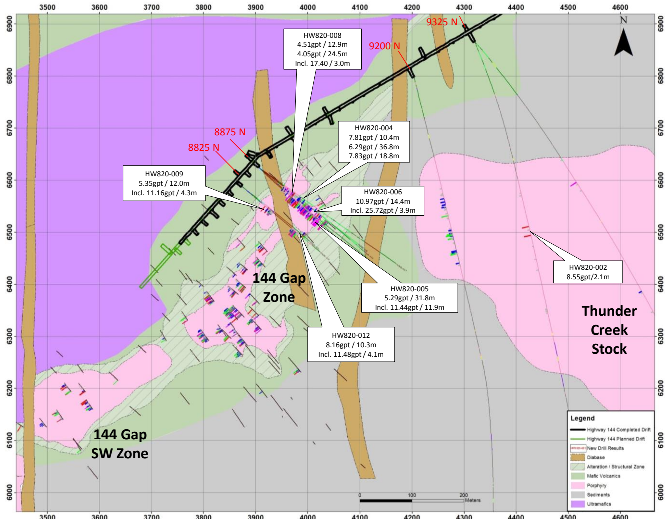
Figure 1. Plan View – 840M Level Showing 144 Exploration Drifts and First 10 Underground Drill Holes
