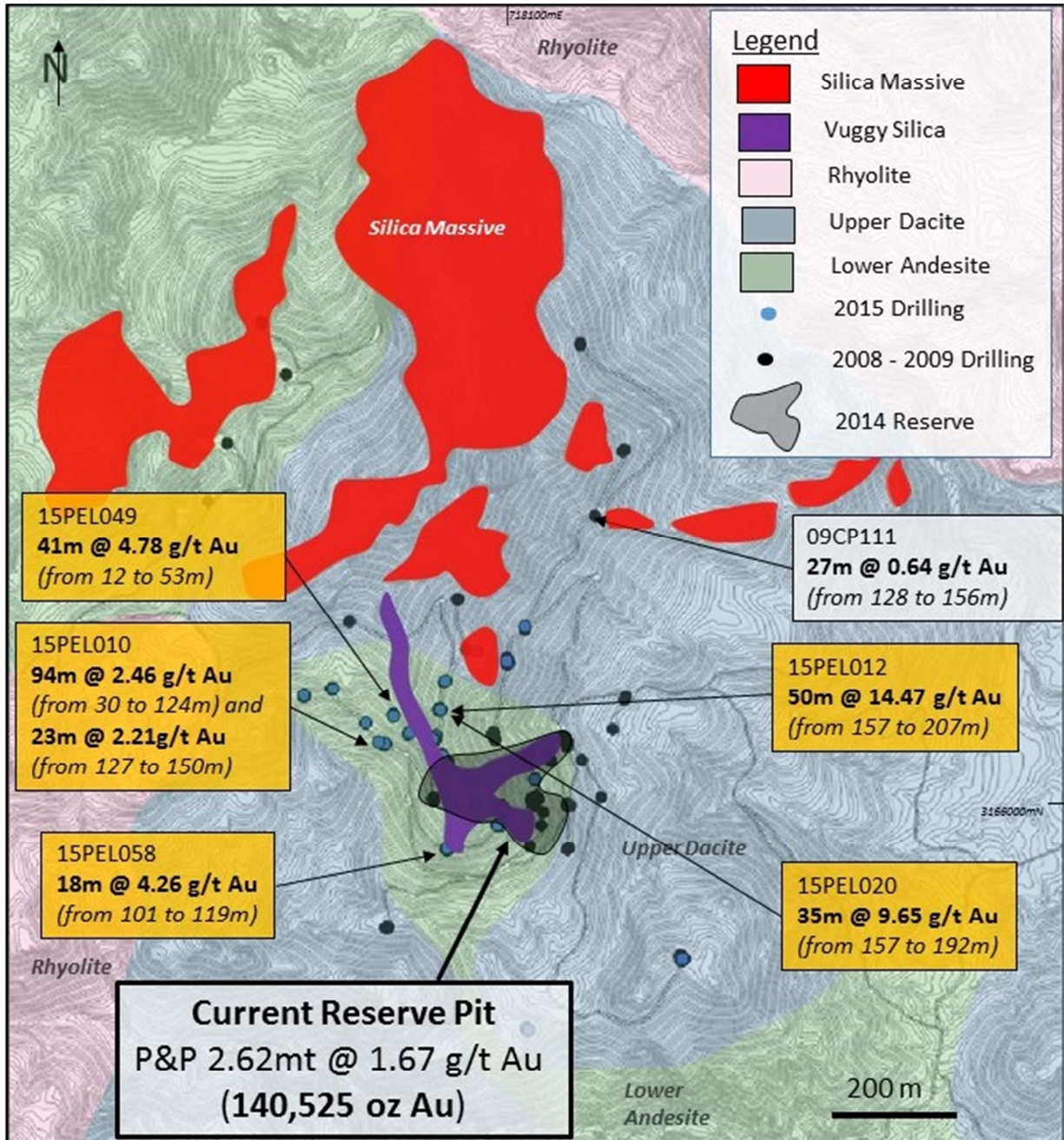
Figure 1: Cerro Pelon Project – Simplified Geology Map with Intercepts
