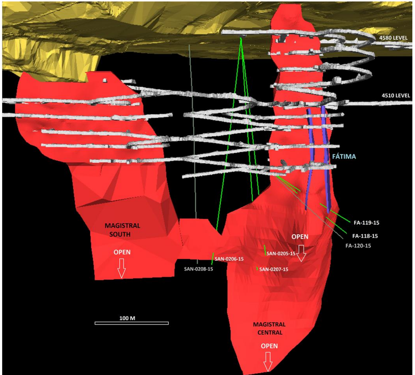
Figure 2: Looking west showing Magistral Central (MC), Magistral South (MS) and Fatima zones (illustrative only) deposits with drill holes location.
