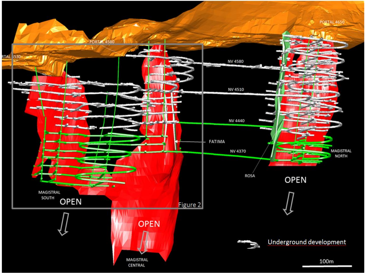
Figure 1: Looking west showing from left to right: Magistral South (MS), Magistral Central (MC), deposits, Fatima and Rosa zones (illustrative only) and Magistral North (MN) at the Santander Zinc Mine in Peru.
