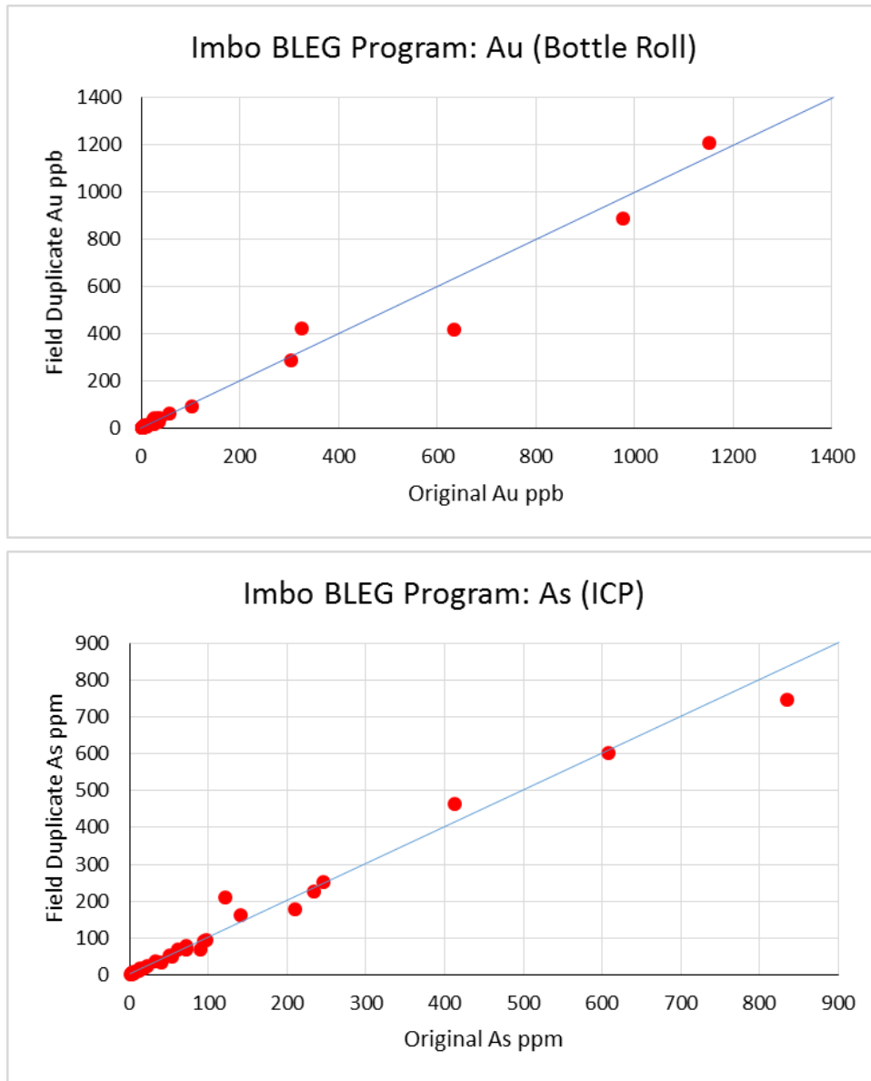
Figure 1 Original Samples v. Field Duplicates (Au & As). Theoretical correlation line shown in blue.
