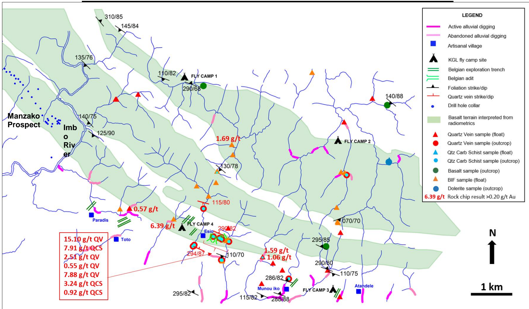
Figure 4 Map of the Imbo Licence (PE9691) east of the Imbo River showing rock chip sampling results and location of artisanal and colonial workings (QV = Quartz Vein, QCS = Quartz-carbonate Schist).
