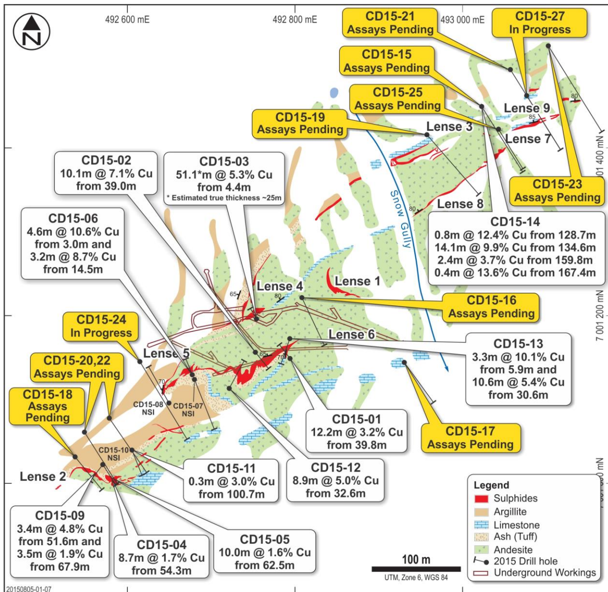
Figure 1. Geology around the nine known lenses of mineralisation at the Caribou Dome Copper Project, together with surface projections of underground development and locations of Coventry's drill holes with analytical results received to date. The surface traces of, and assay results from, the 112 holes drilled prior to Coventry's involvement in the Project are not shown on this plan.
