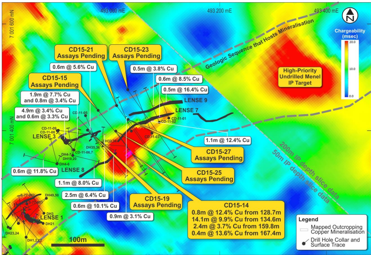
Figure 2. Combination of 50-metre and 200-metre “depth slices” of inverted IP chargeability data at the Lense 7/8 and Menel Targets – showing the chargeability of the modelled source of IP anomalies, 50 and 200 metres below the surface respectively, together with previous drilling in the vicinity.
