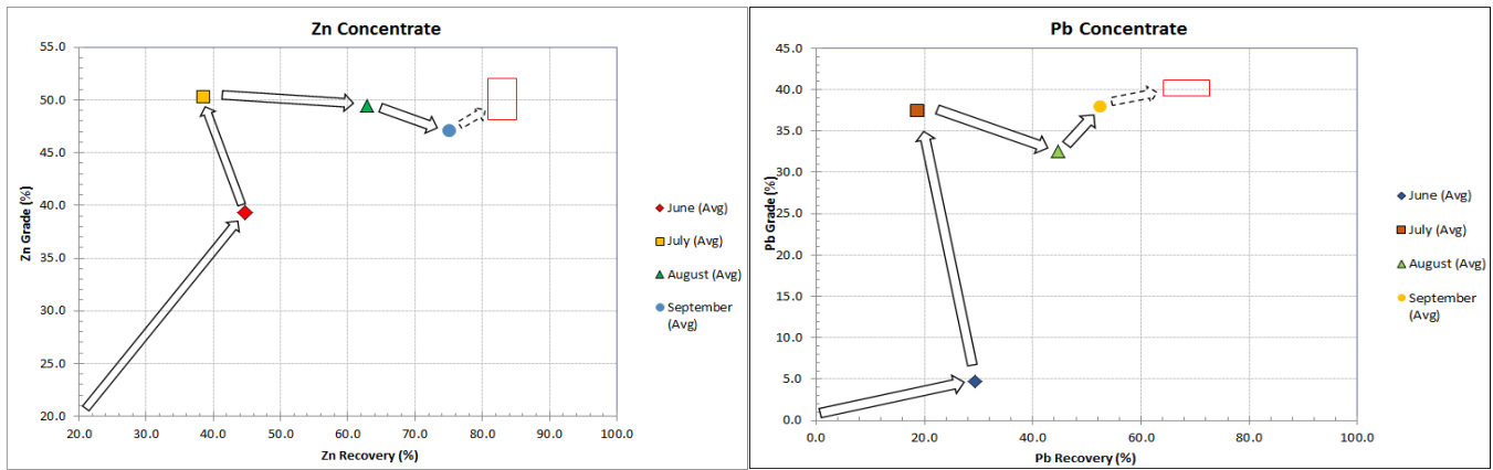
Figure 1: Graphs of Zn concentrate grade (left) and Pb concentrate grade (right) versus circuit recovery from June through September. Red box indicates Caribou target grade – recovery design window.
