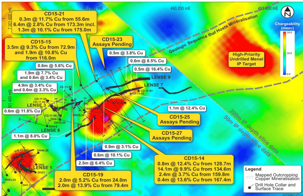
Figure 1. Combination of 50-metre and 200-metre “depth slices” of inverted IP chargeability data at the Lense 7/8 and Menel Targets – showing the chargeability of the modelled source of IP anomalies, 50 and 200 metres below the surface respectively, together with previous (white text boxes) and recent (yellow text boxes) drilling results in the vicinity.
