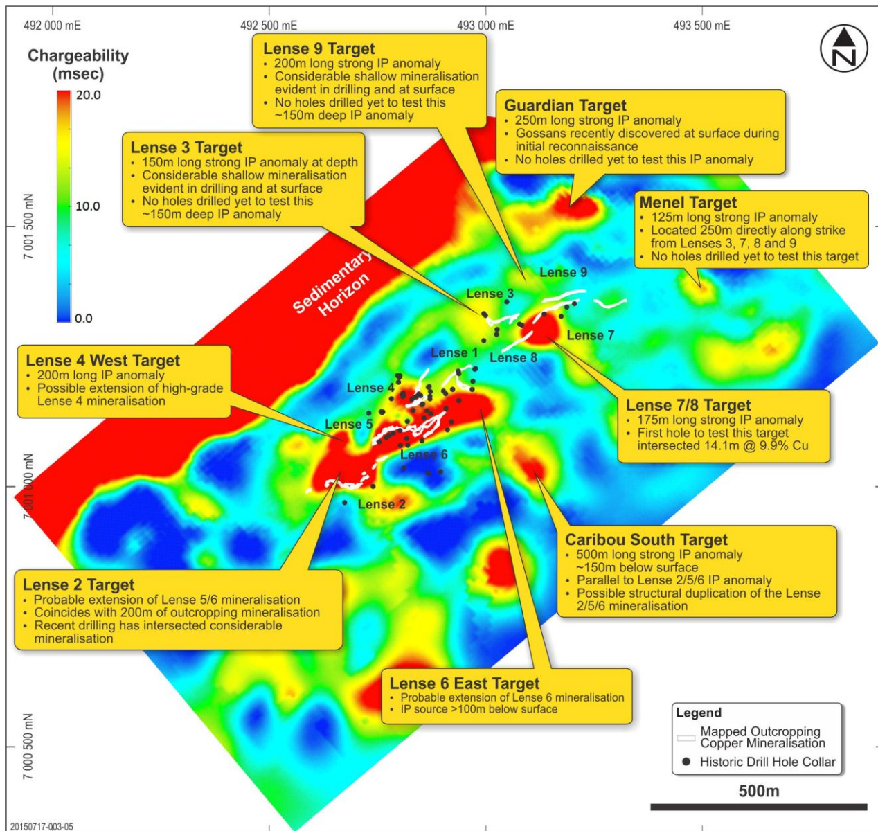
Figure 3. “100-metre depth slice” of inverted 3DIP chargeability data – showing the chargeability of the modelled source of 3DIP anomalies, 100 metre surface, together with labels highlighting higher-priority targets that will be evaluated further. (It is noted that the sources of some of the highest priority modelled to be greater than and less than 100 metres deep – so not all targets appear as intense anomalies in the 100m depth slice plan above).
