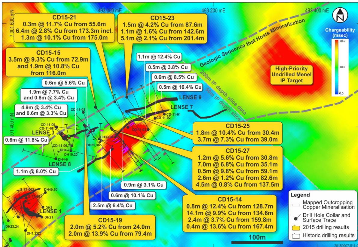
Figure 1. Combination of 50-metre and 200-metre “depth slices” of inverted IP chargeability data at the Lense 7/8 and Menel Targets – showing the chargeability of the modelled source of IP anomalies, 50 and 200 metres below the surface respectively, together with previous (white text boxes) and recent (yellow text boxes) drilling results in the vicinity.
