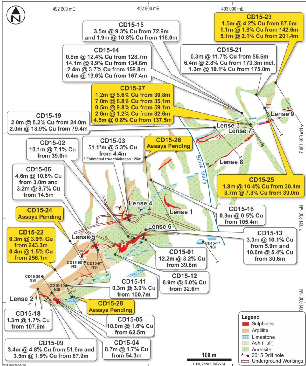
Figure 4. Geology around the nine known lenses of mineralisation at the Caribou Dome Copper Project, together with surface projections of underground development and locations of Coventry's drill holes with analytical results received to date. The surface traces of, and assay results from, the 112 holes drilled prior to Coventry's involvement in the Project are not shown on this plan.
