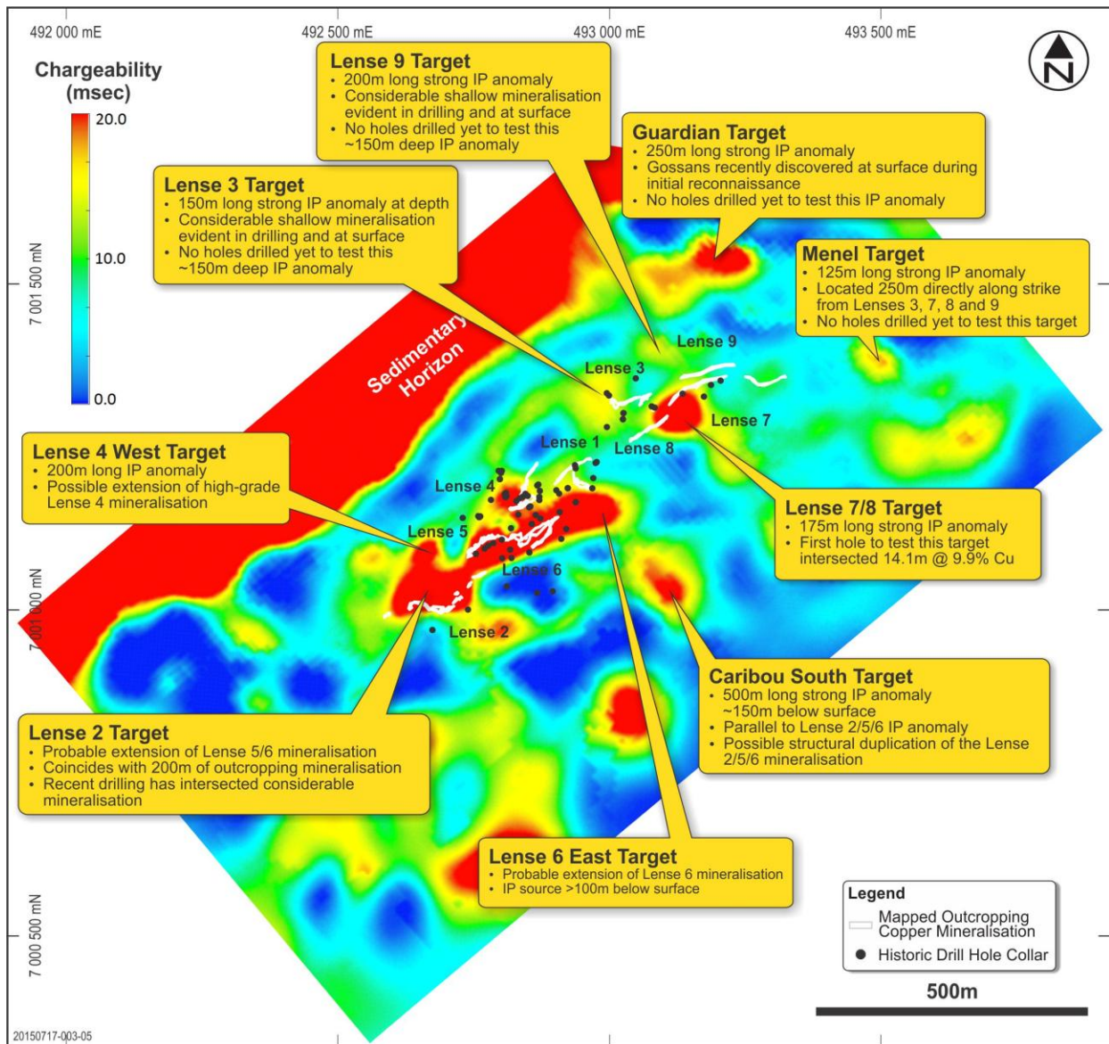
Figure 5. "100-metre depth slice" of inverted 3DIP chargeability data – showing the chargeability of the modelled source of 3DIP anomalies, 100 metres below the surface, together with labels highlighting higher-priority targets that will be evaluated further. (It is noted that the sources of some of the highest priority targets are modelled to be greater than and less than 100 metres deep – so not all targets appear as intense anomalies in the 100m depth slice plan above).
