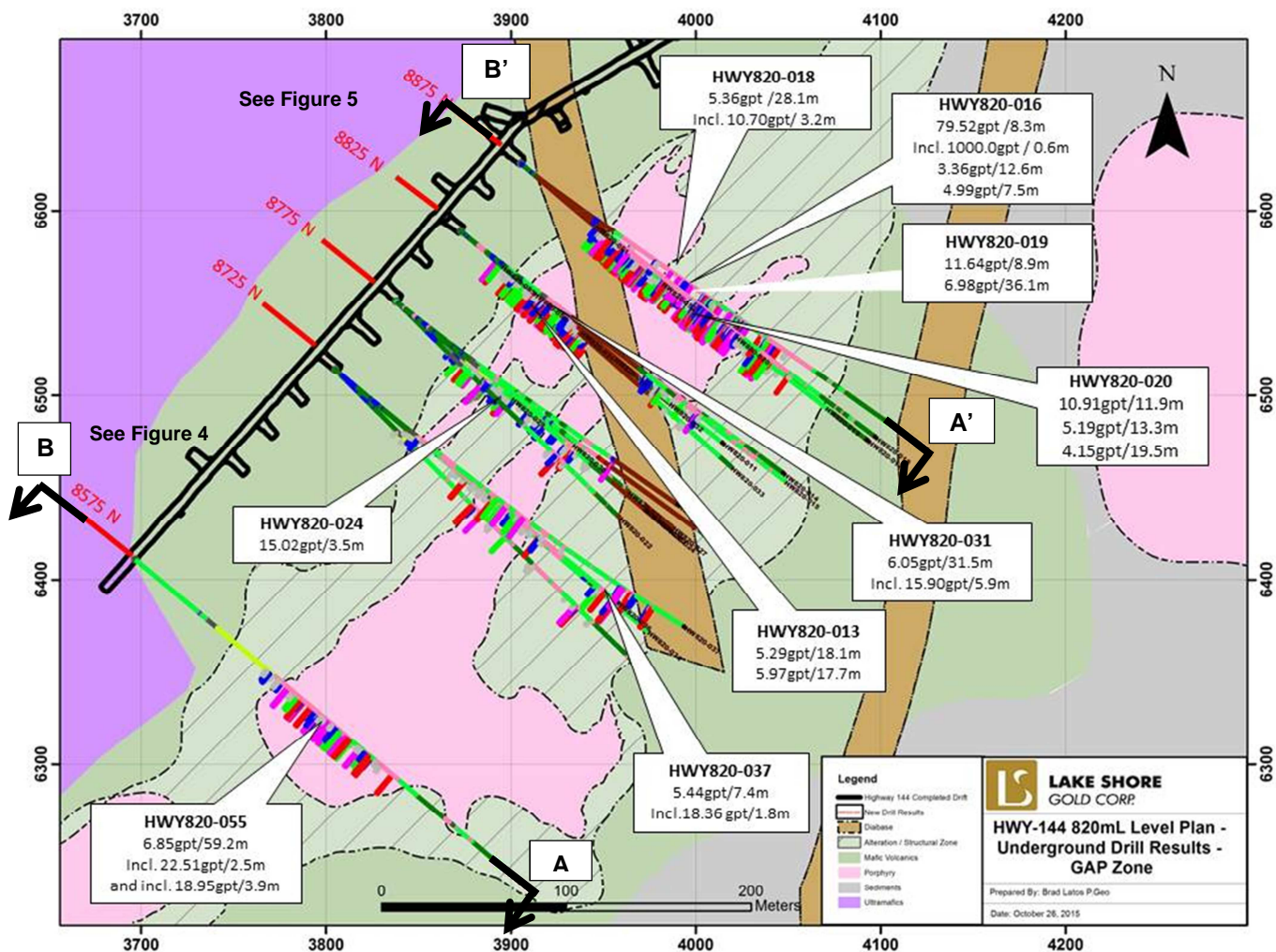
Figure 3. Plan View – 144 Gap Zone showing new underground drill holes
