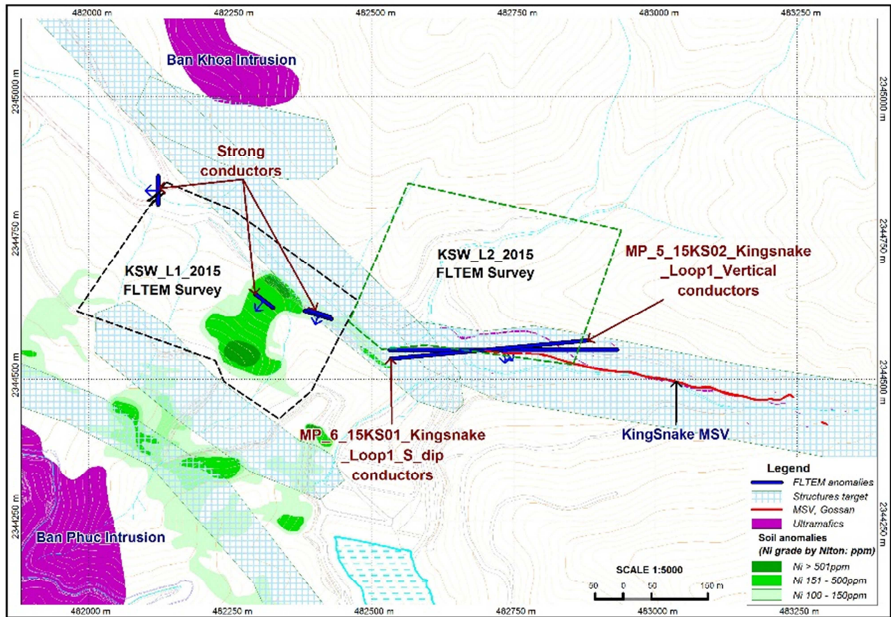
Figure 2: FLTEM Overlay with nickel and copper soils & conceptual targets Conceptual target (blue hatched); identified conductors (solid blue); soil anomalies (green)
