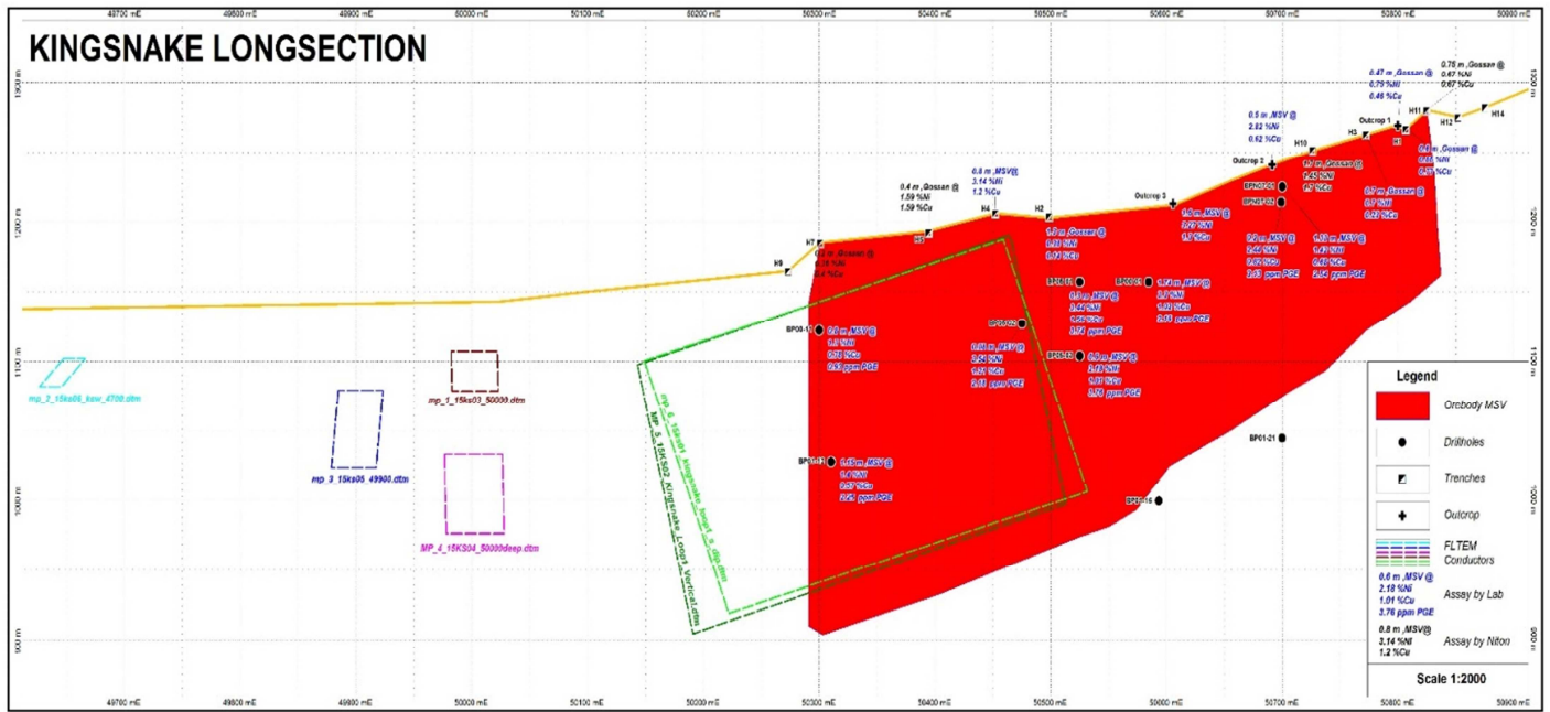
Figure 3: Kingsnake Long-section showing identified electromagnetic conductors
