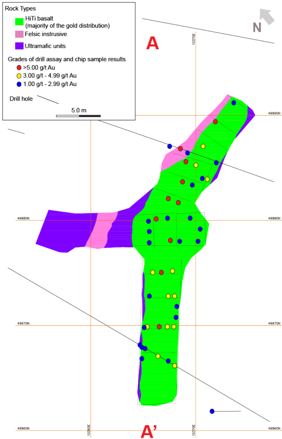
Figure 2: Plan View Section of 489 Stope – 244-metre level
