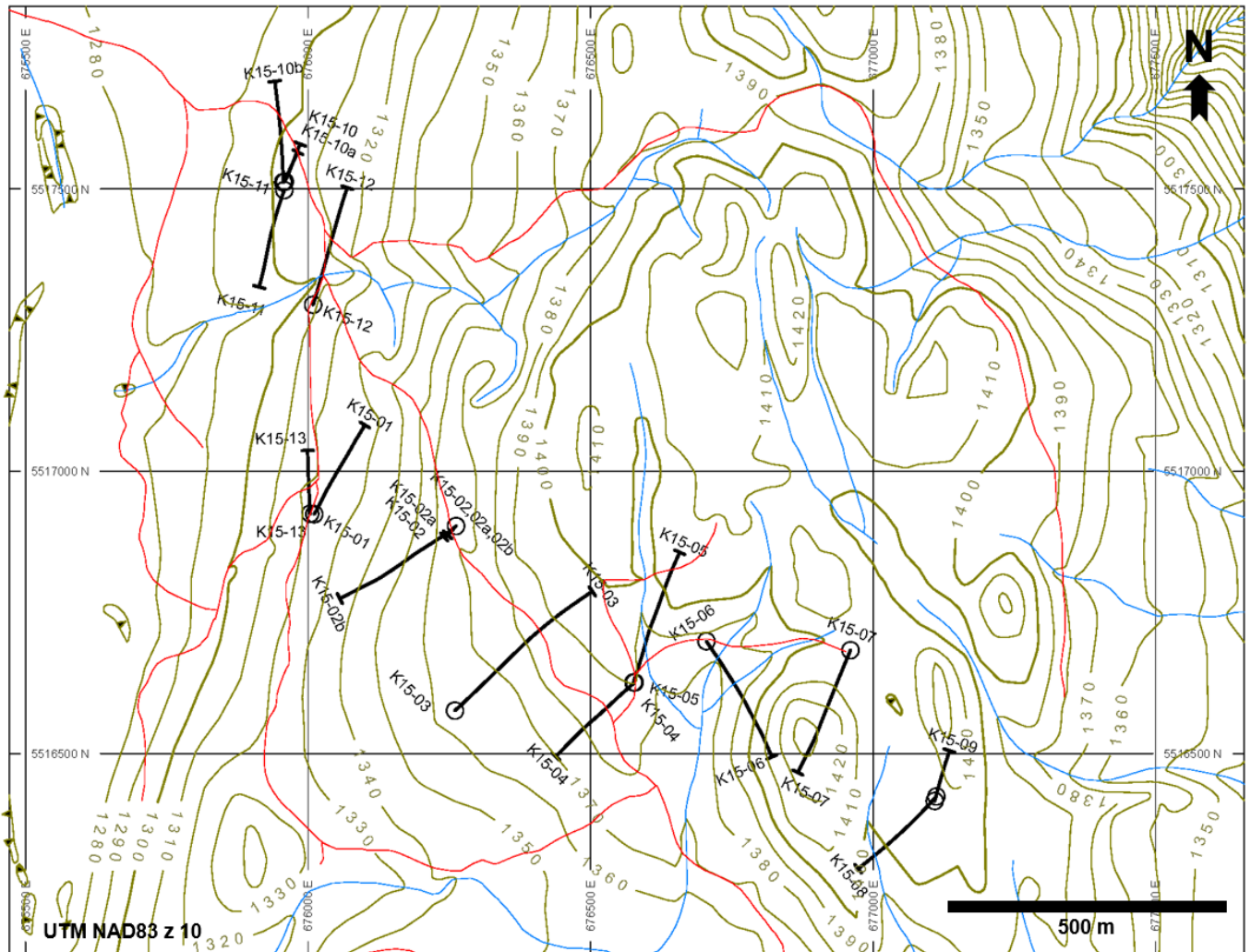
Figure 2: 2015 drill collars on the Ketchan prospect, Aspen Grove Project.
