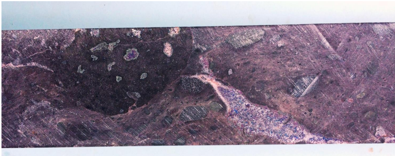
Figure 3: Coarse bornite replacing clasts and in veins, within diamictite, in DKMC_DD996 at a depth of 353.50 metres.
