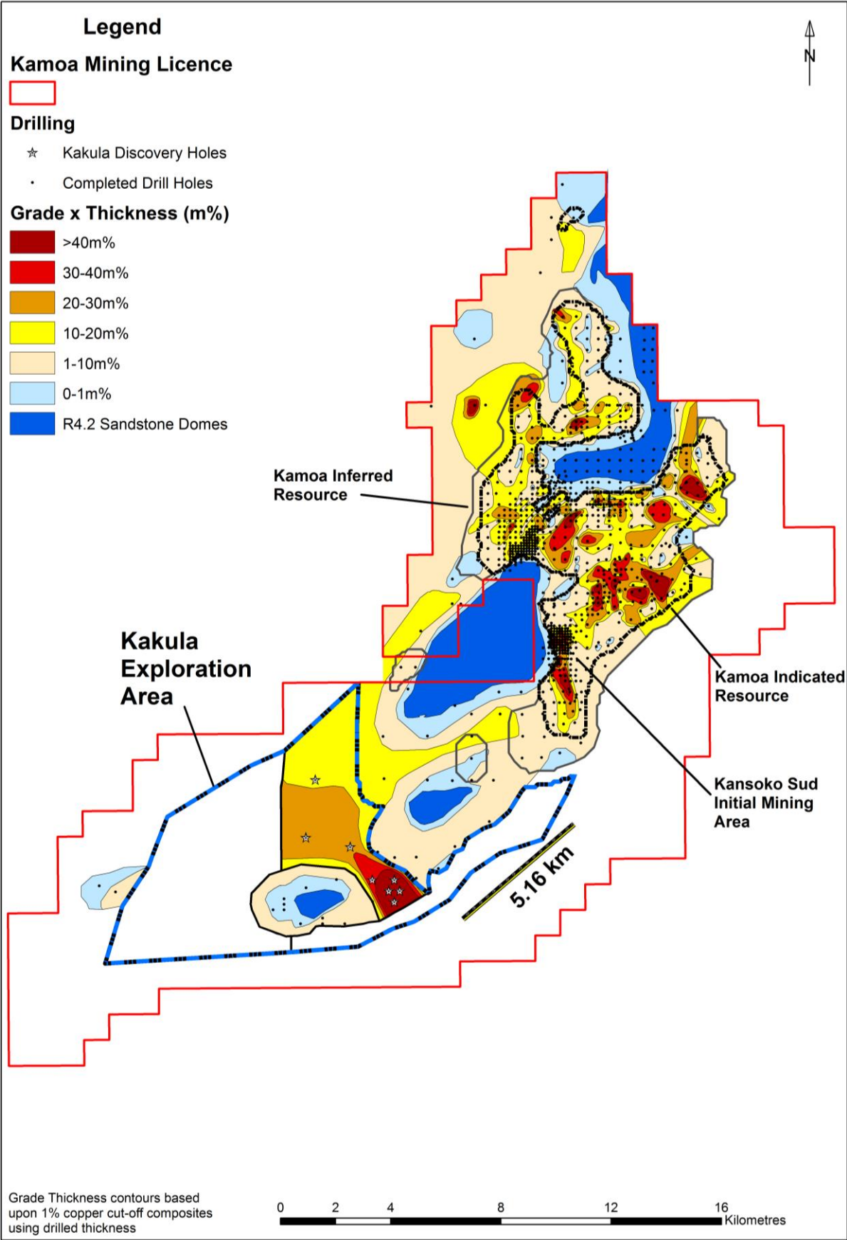
Figure 5: Kamoa Mining Licence area showing grade-thickness contours across the Kamoa Copper Project and the area of the Kakula Discovery holes.
