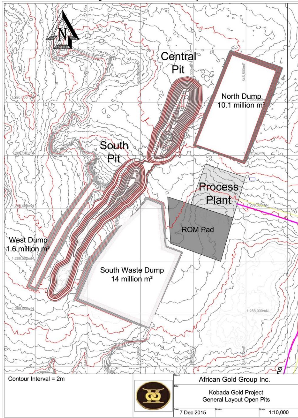
Figure 1 – General Mine Layout
