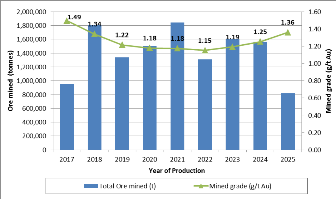
Figure 2 - Ore mined by year and average grade
