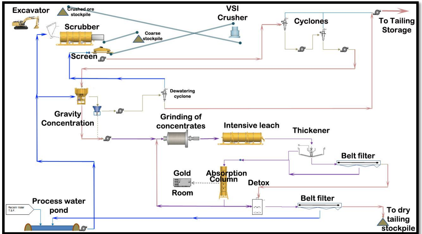
Figure 4 – Simplified Processing Flow Sheet
