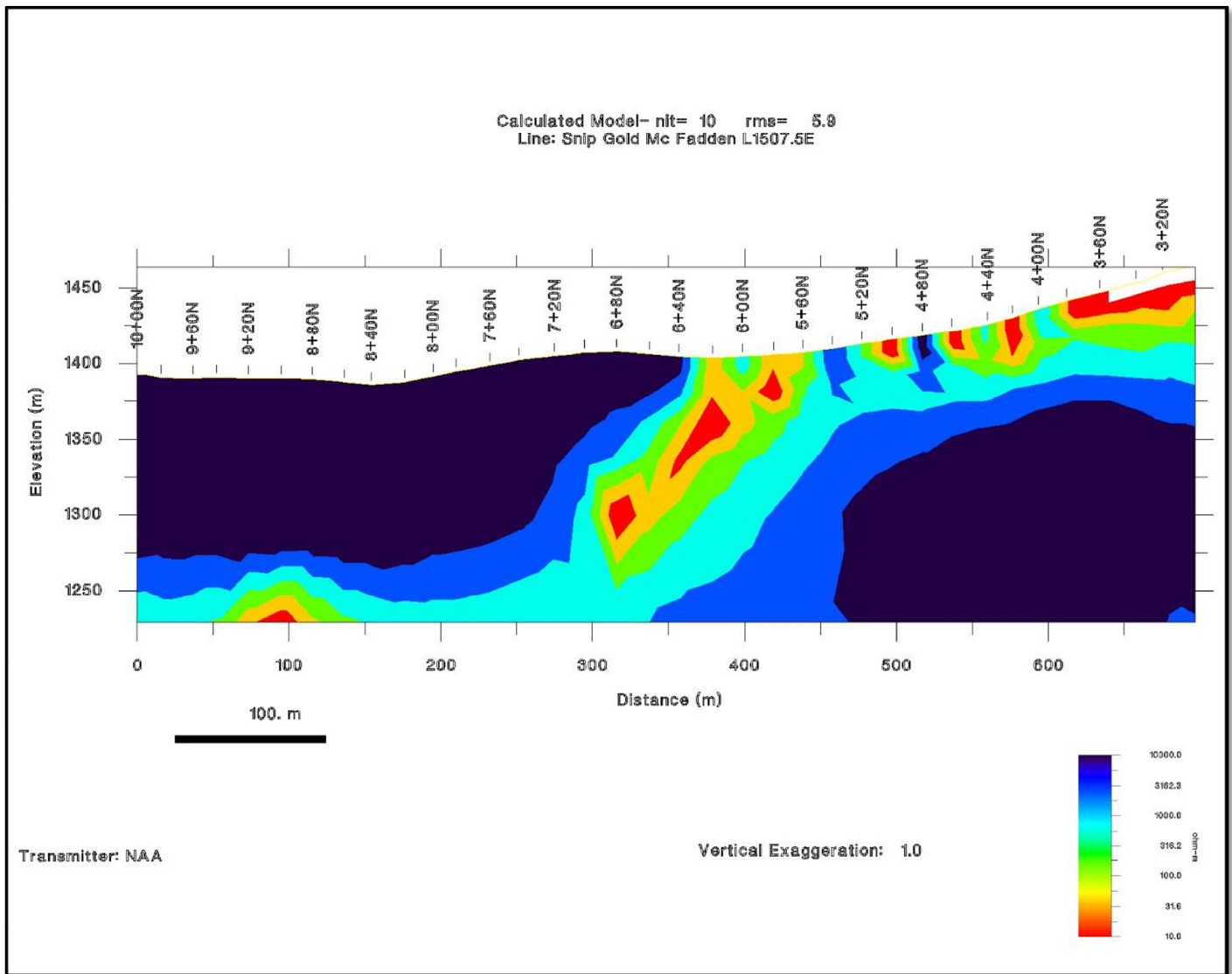
Figure 5. Displays the profile for the 2015 Cutler Maine (NAA) modeled data for section L1507.5E, the vertical cross section view looks easterly in an upslope direction. The surface trace of this profile is shown on figure 3. The areas noted from green to red show areas of higher conductivity and are interpreted to be the possible source for the high-grade boulders at McFadden.
