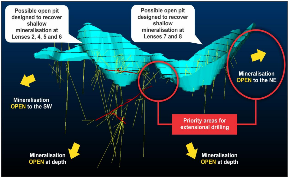
Figure 1. Results from initial open pit mining studies, indicating two adjacent open pits are currently optimal, potentially because very limited drilling has been undertaken previously between Lenses 4, 5 and 6 (LHS) and Lenses 7/8 (RHS). Extensions of mineralisation in this area will be targeted during the Company's next drilling program. Traces of all drill holes are illustrated in yellow. Historic underground exploration development is highlighted in red.
