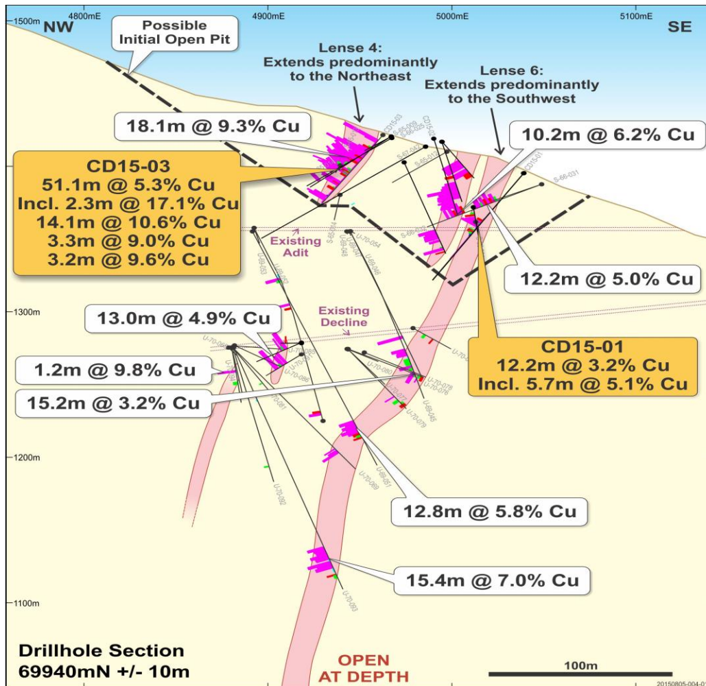
Figure 2. Cross Section 69940N showing mineralisation at Lenses 4 and 6 and a possible open pit that might be used to recover the thick, shallow, high-grade mineralisation within approximately 100 metres of surface. Considerable thick, high-grade mineralisation extends well below the conceptual open pit. This deeper mineralisation may be recoverable with underground mining methods.
