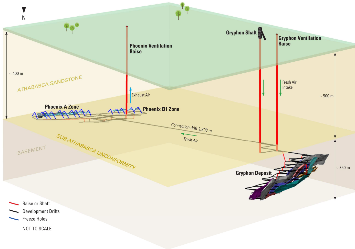
Figure 1: Wheeler River Underground Schematic
