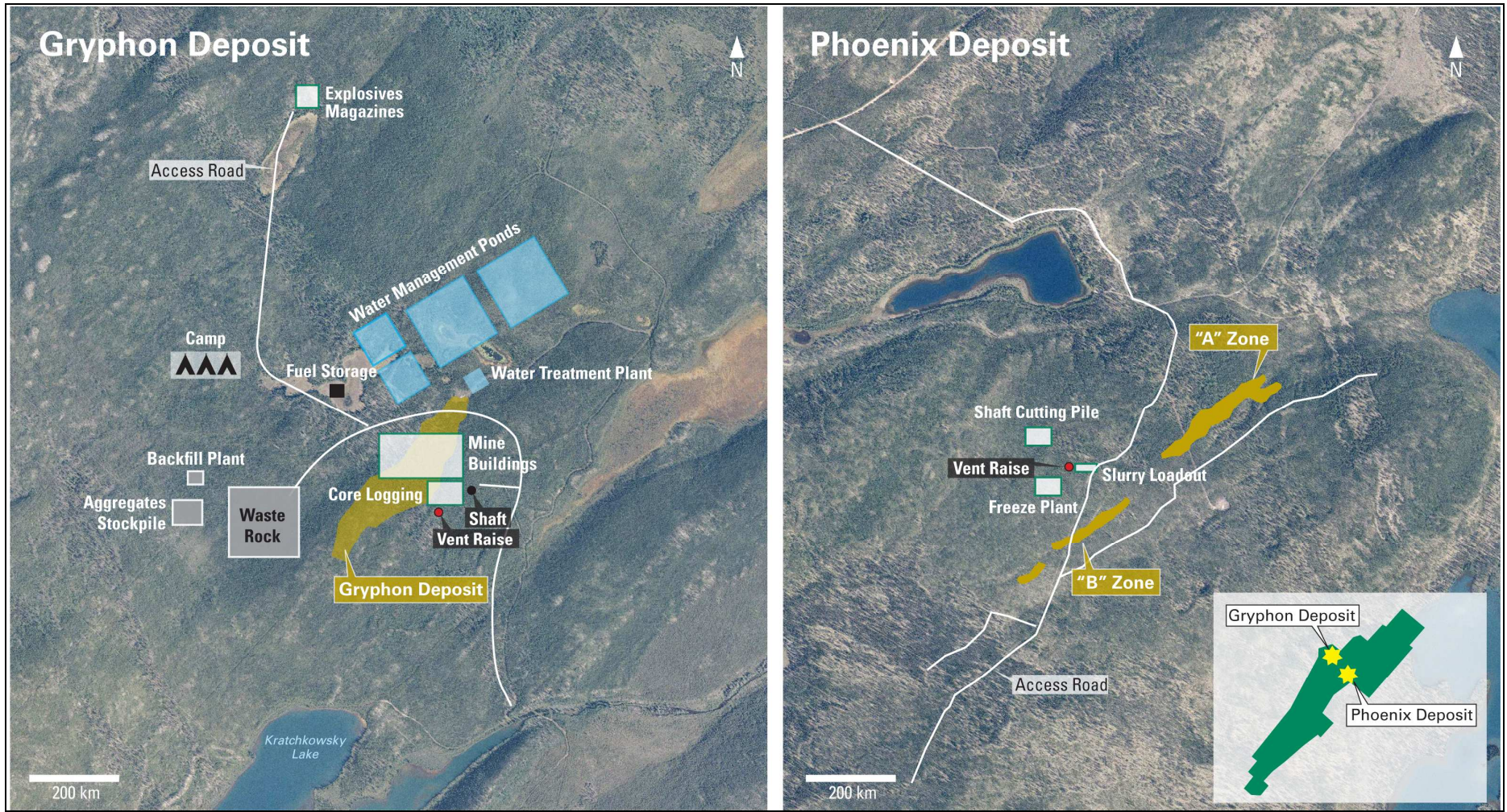
Figure 2: Wheeler River Surface Schematic
